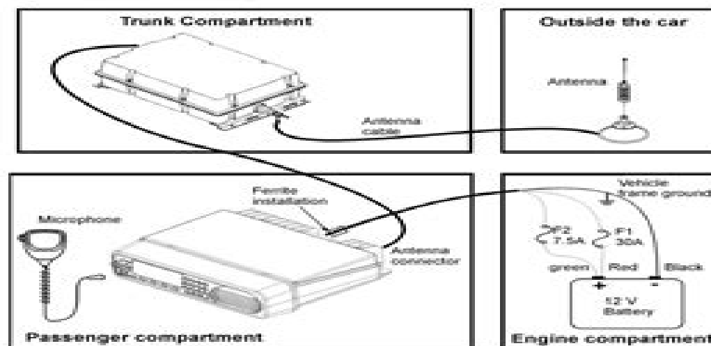
Figure 3: Front Model Installation Diagram
