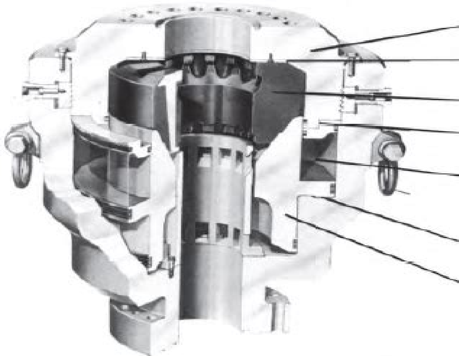
Hydril GX Annular
