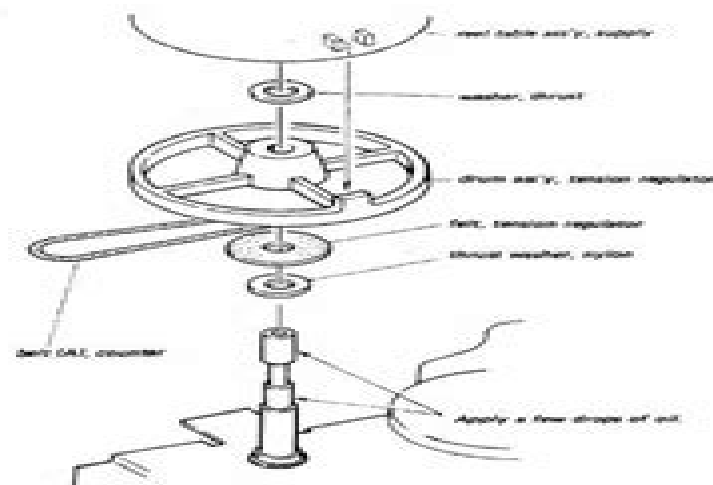
Fig. 2 Tension regulator drum installation
