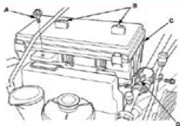
Fig. 57: Identifying Under-Hood Fuse/Relay Box Bolt And Clamps Courtesy of AMERICAN HONDA MOTOR CO., INC.
