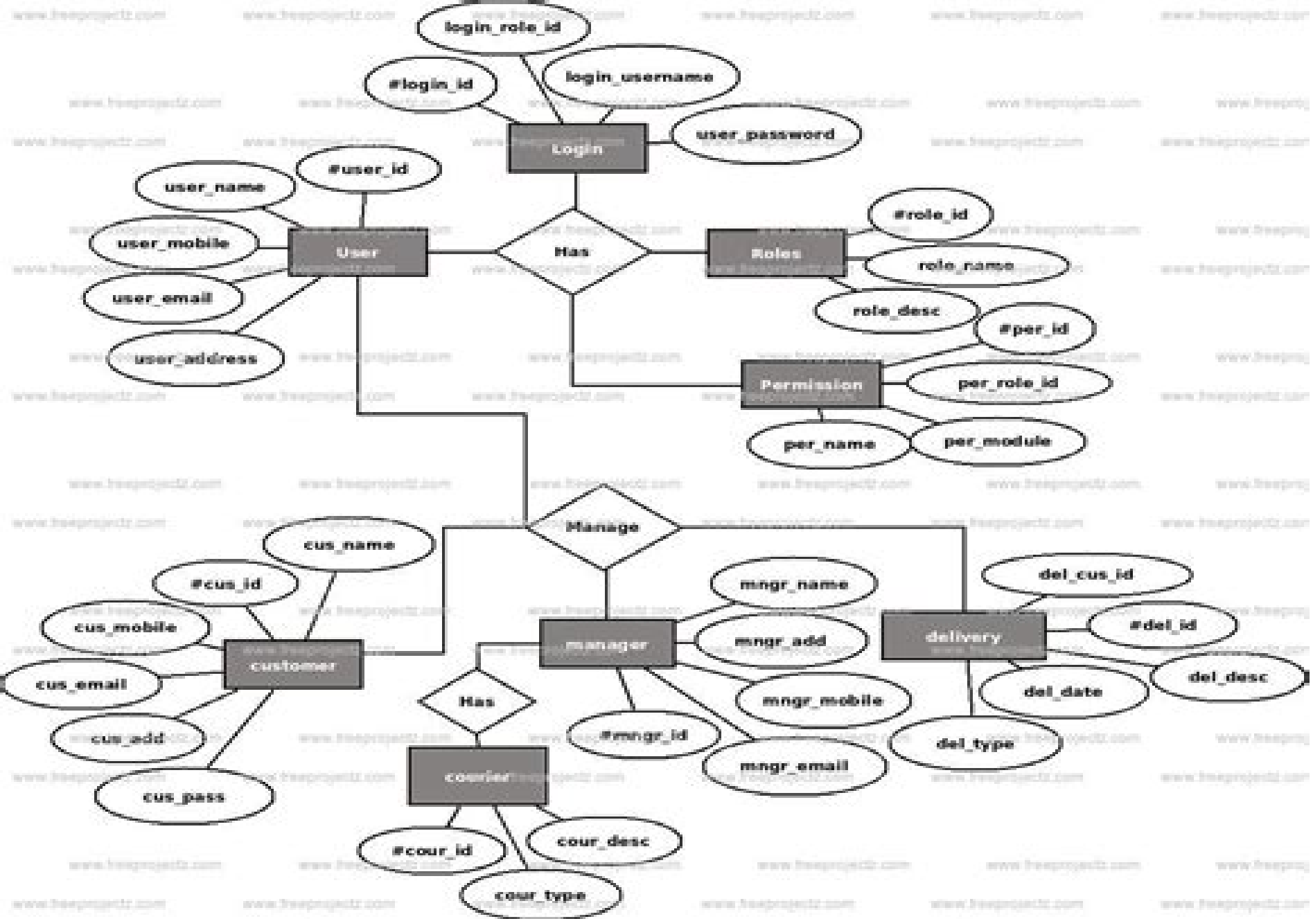
ER Diagram For Courier Management System
