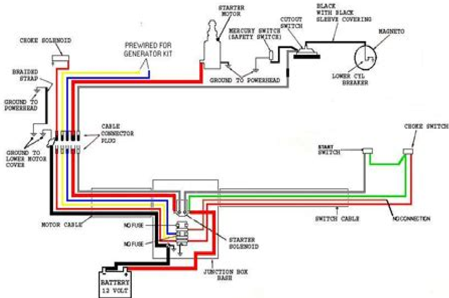
WIRING DIAGRAM FOR 1957 35 HORSEPOWER MODEL
