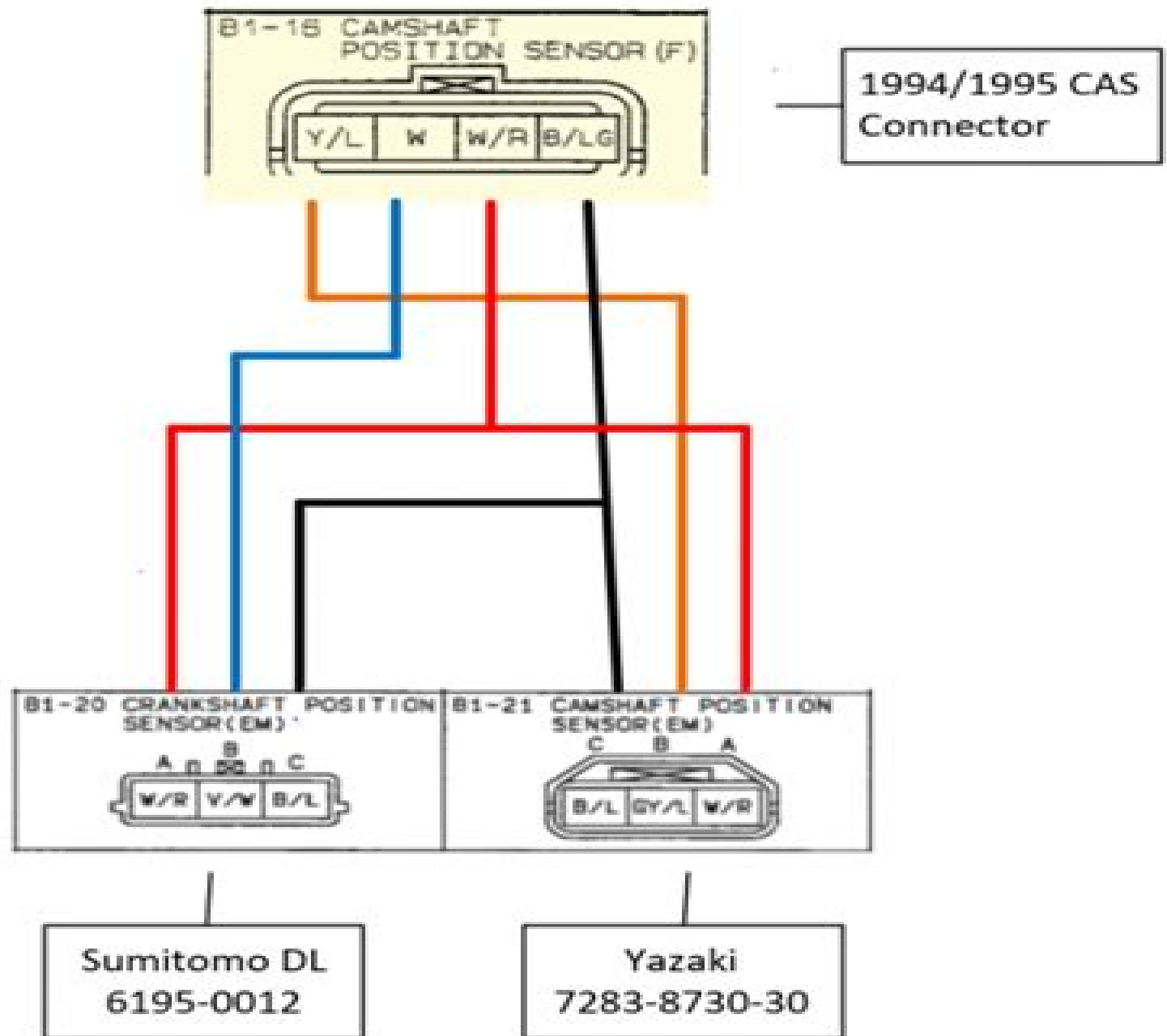
VVT Engine Crank/Cam Sensors
