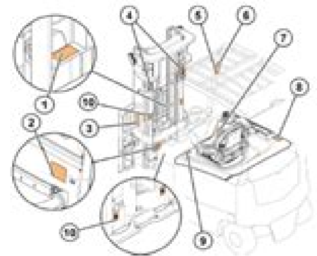
Figure 1: Parts and elements of the truck overview
