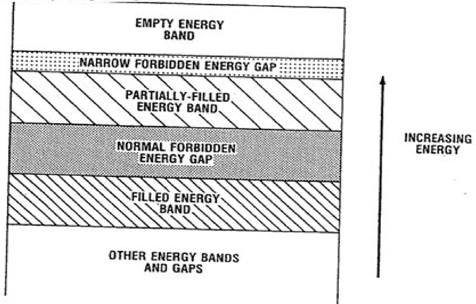
Figure 3-2. Relevant energy levels in gallium arsenide.
