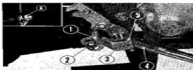
① Brake pedal spring ③ 10 mm nut ② Tensioner lock arm ④ Brake pedal ⑤ Tensioner lock arm mounting bolt ⑥ Brake adjuster nut Fig. 14
